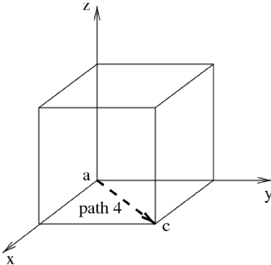
Figure 1: Figure 2: d\vec{r} along path 4
